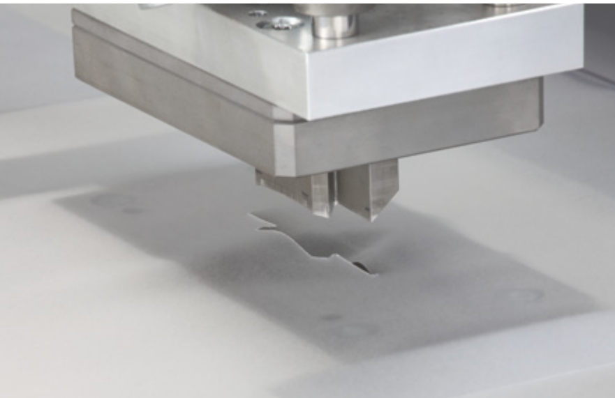
By using high-precision stamping tools optional cut-outs, for example cable feeds for the backsheet foil, are possible at any location.
